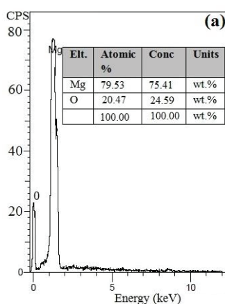
MgO
